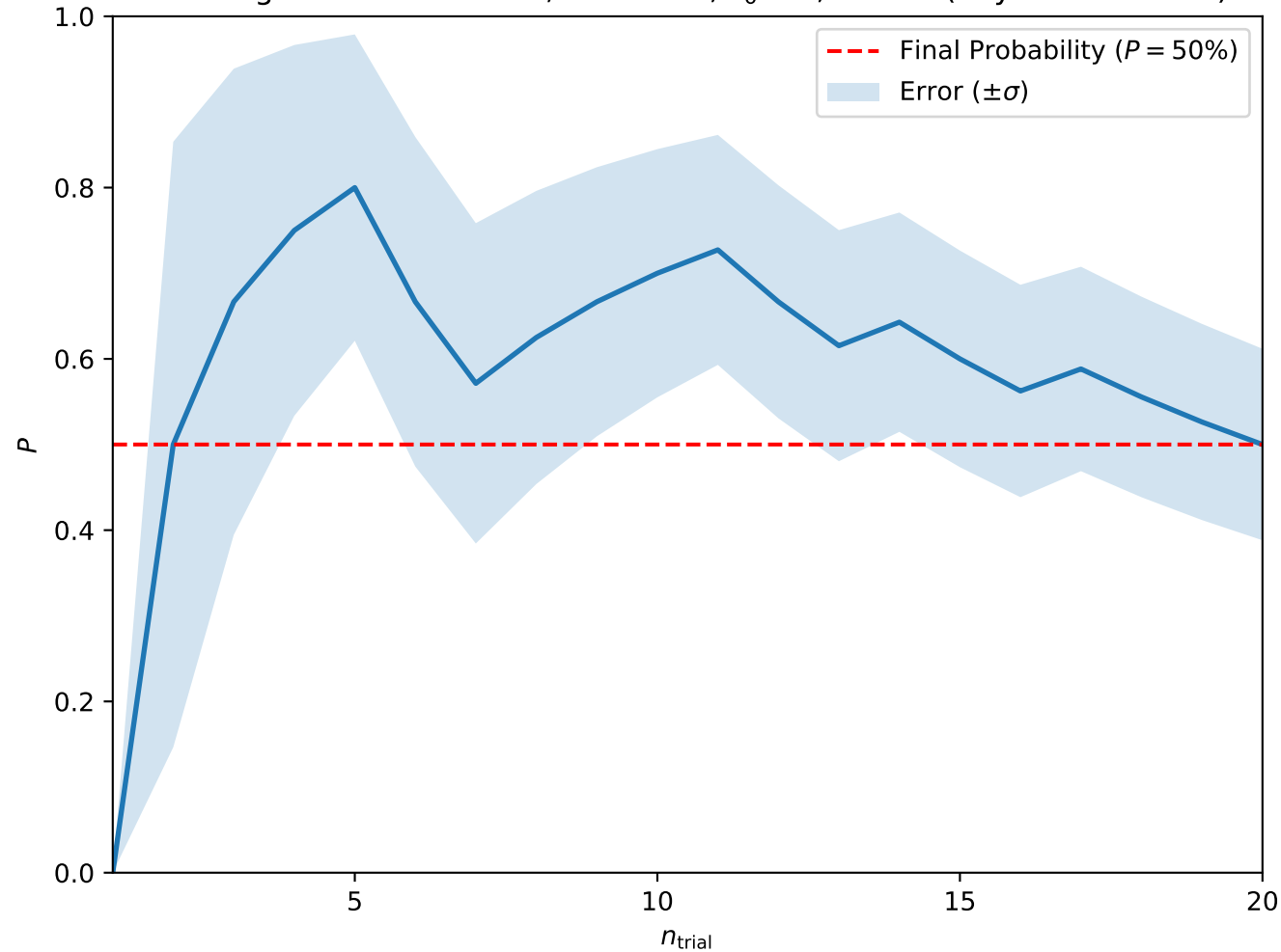
Convergence at A = 0.275, H = 0.275, T_0 = 3, w = 10 (Skyrmion Lattice)
