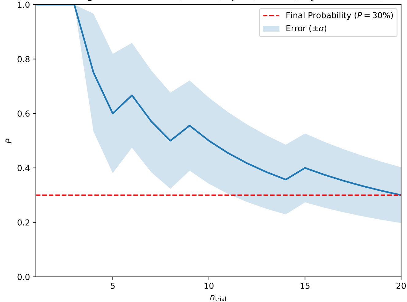
Convergence at A = 0.275, H = 0.3, T_0 = 3, w = 10 (Skyrmion Lattice)
