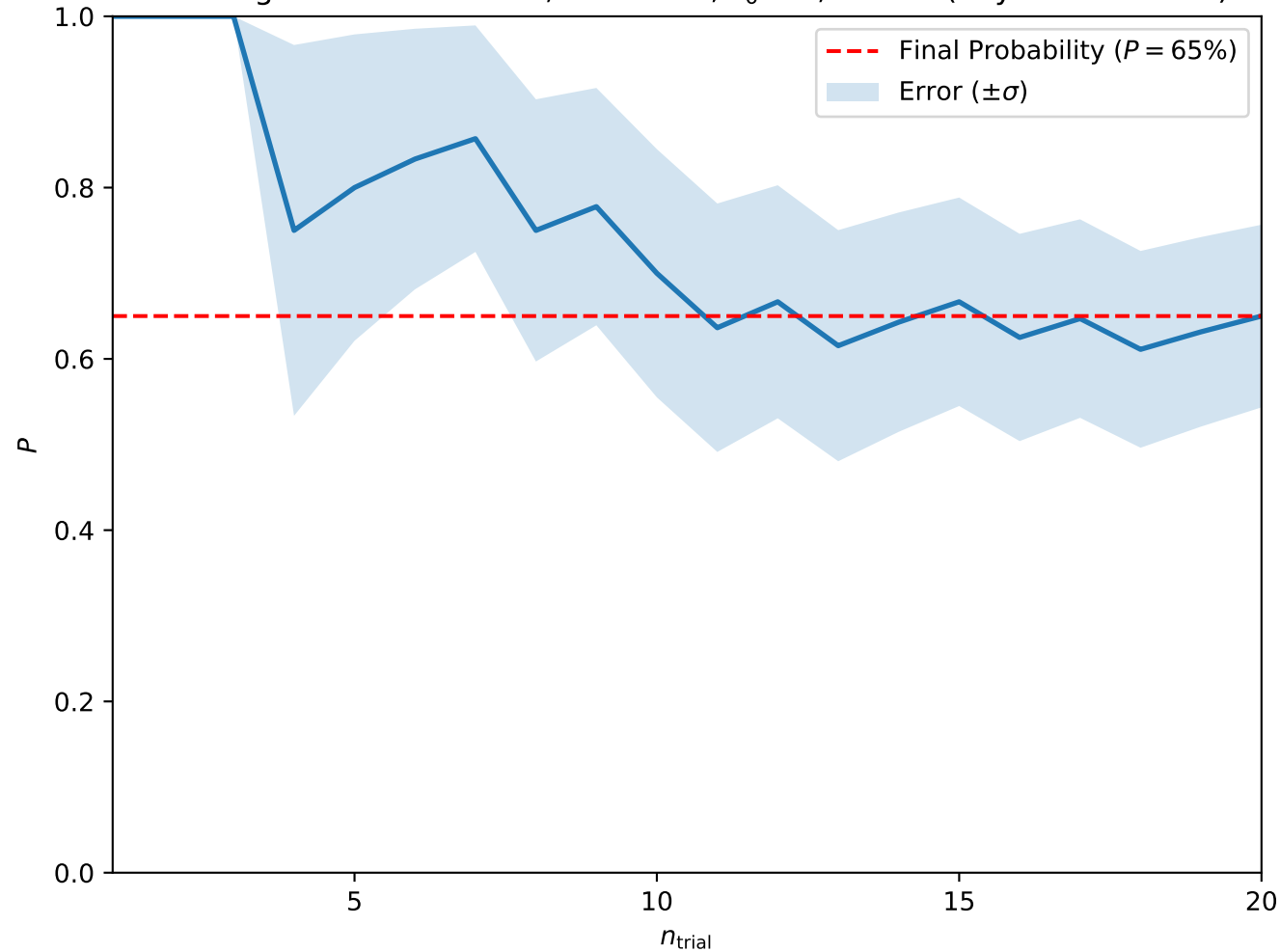
Convergence at A = 0.275, H = 0.325, T_0 = 3, w = 10 (Skyrmion Lattice)
