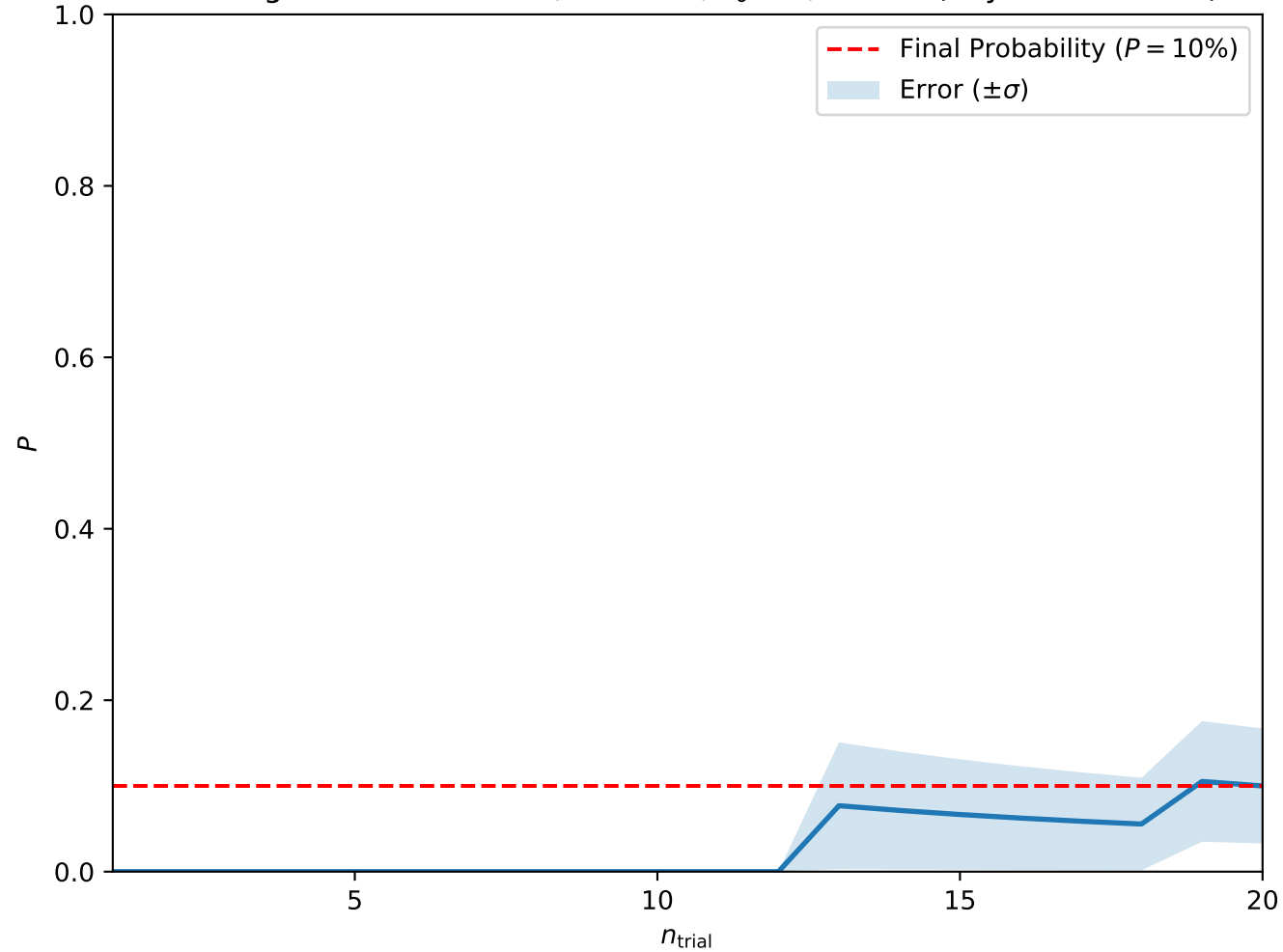
Convergence at A = 0.275, H = 0.35, T_0 = 3, w = 10 (Skyrmion Lattice)
