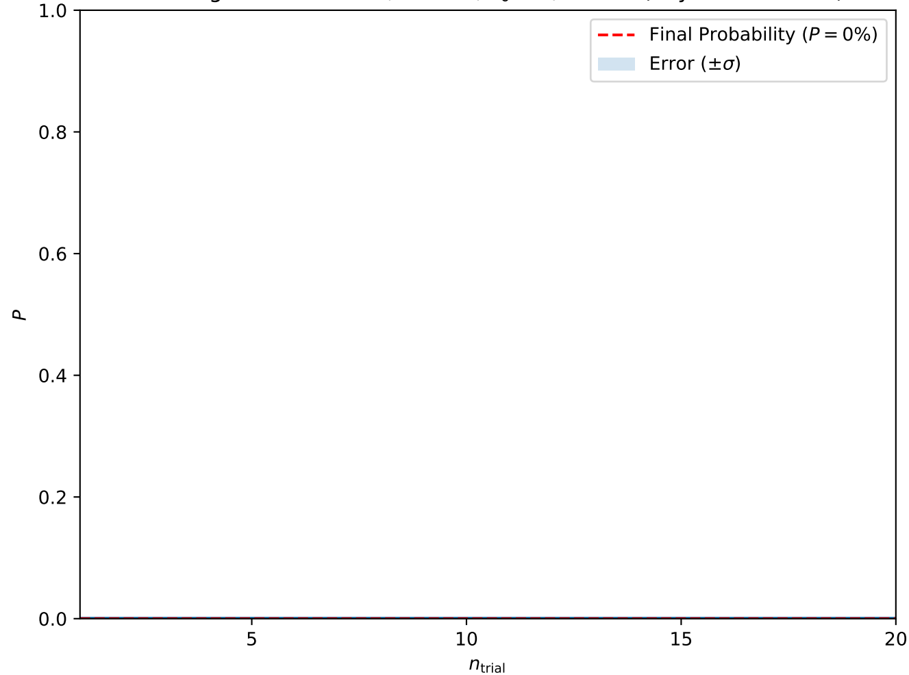
Convergence at A = 0.2, H = 0.2, T_0 = 3, w = 10 (Skyrmion Lattice)
