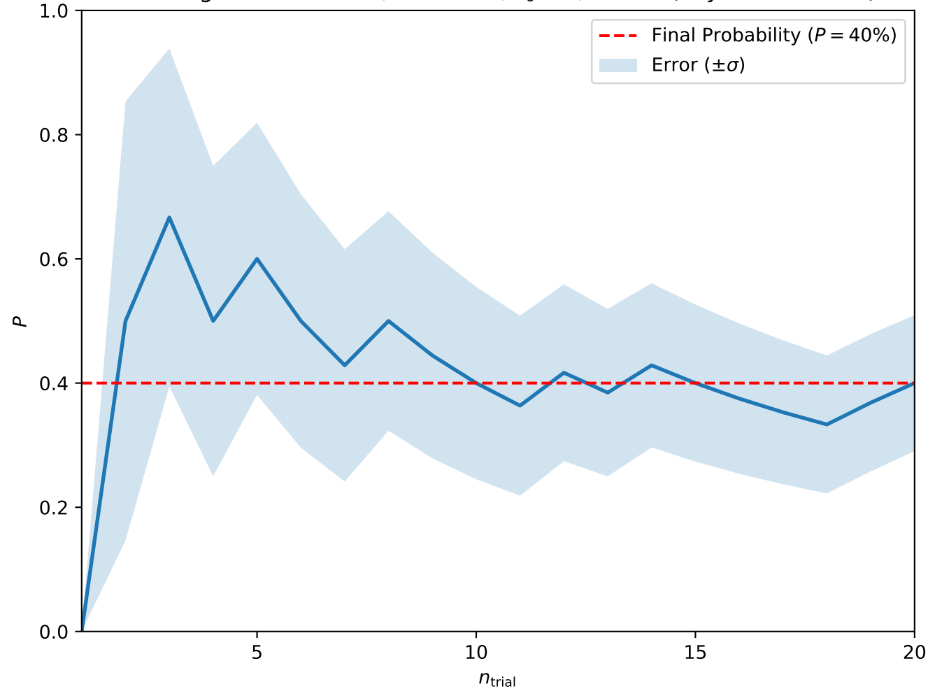
Convergence at A = 0.2, H = 0.275, T_0 = 3, w = 10 (Skyrmion Lattice)
