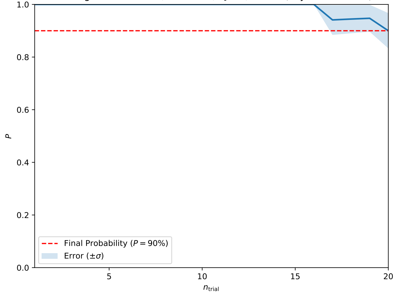
Convergence at A = 0.2, H = 0.325, T_0 = 3, w = 10 (Skyrmion Lattice)
