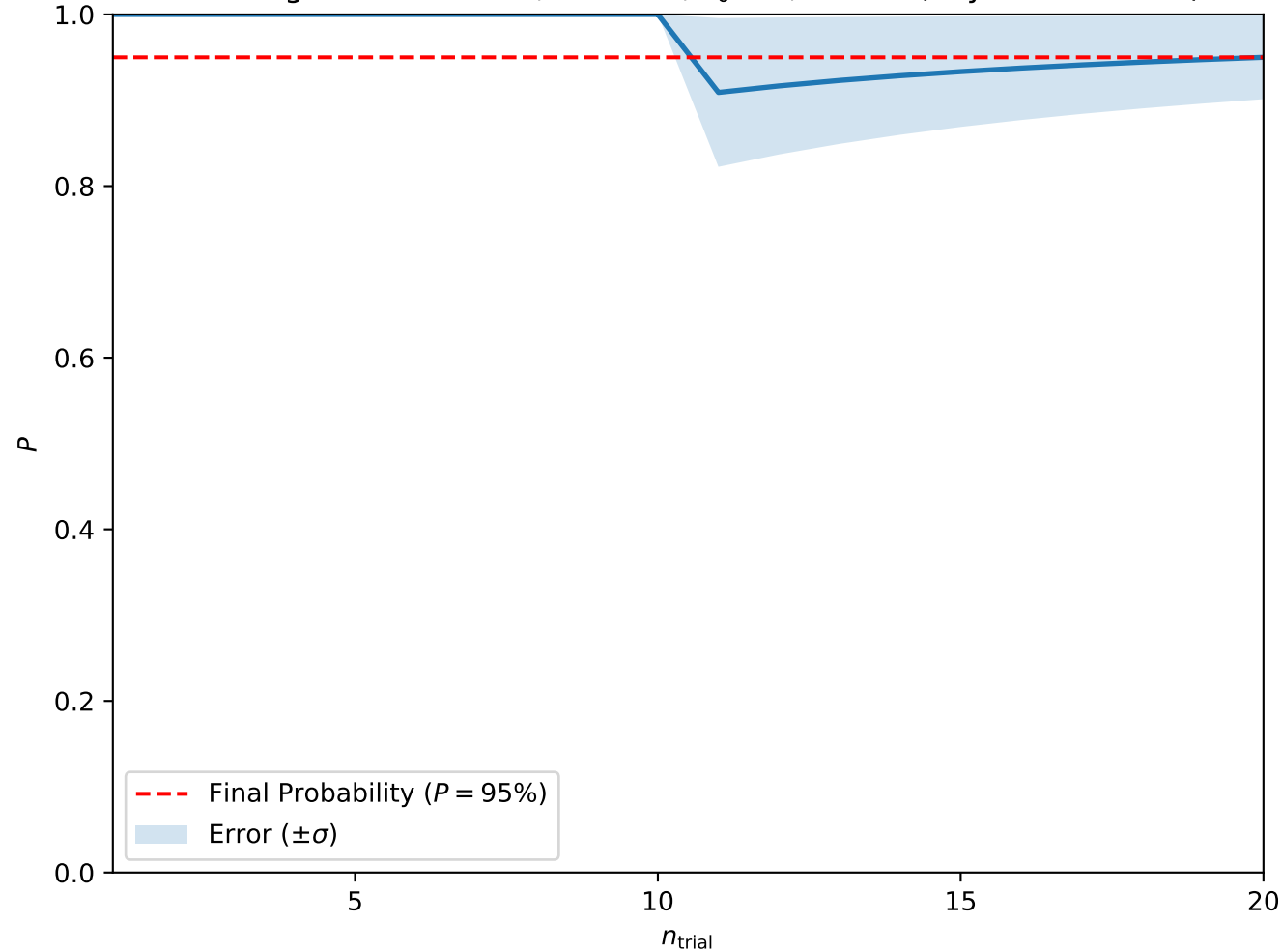
Convergence at A = 0.2, H = 0.35, T_0 = 3, w = 10 (Skyrmion Lattice)
