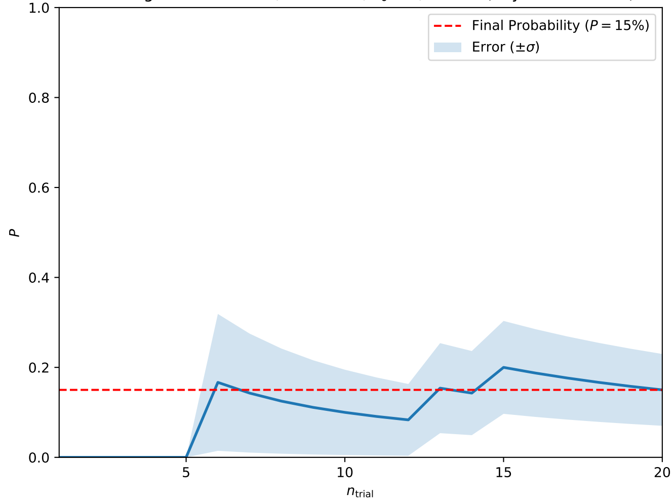
Convergence at A = 0.2, H = 0.425, T_0 = 3, w = 10 (Skyrmion Lattice)
