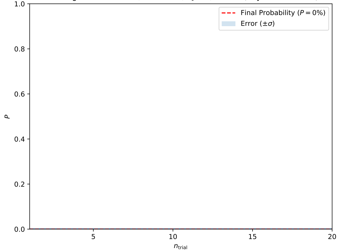
Convergence at A = 0.2, H = 0.525, T_0 = 3, w = 10 (Skyrmion Lattice)
