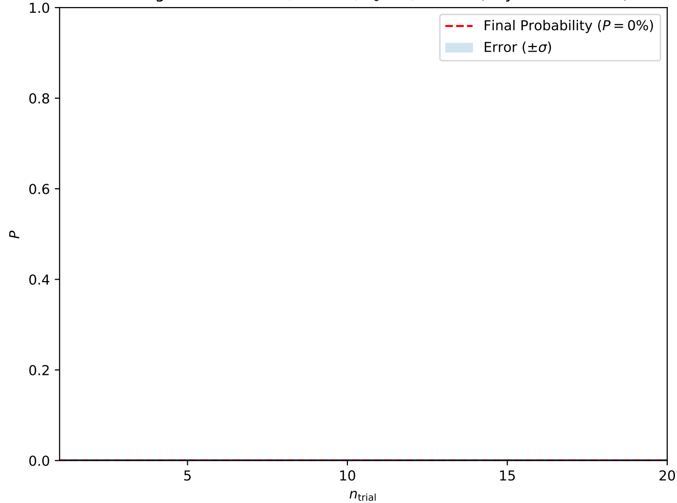
Convergence at A = 0.2, H = 0.6, T_0 = 3, w = 10 (Skyrmion Lattice)
