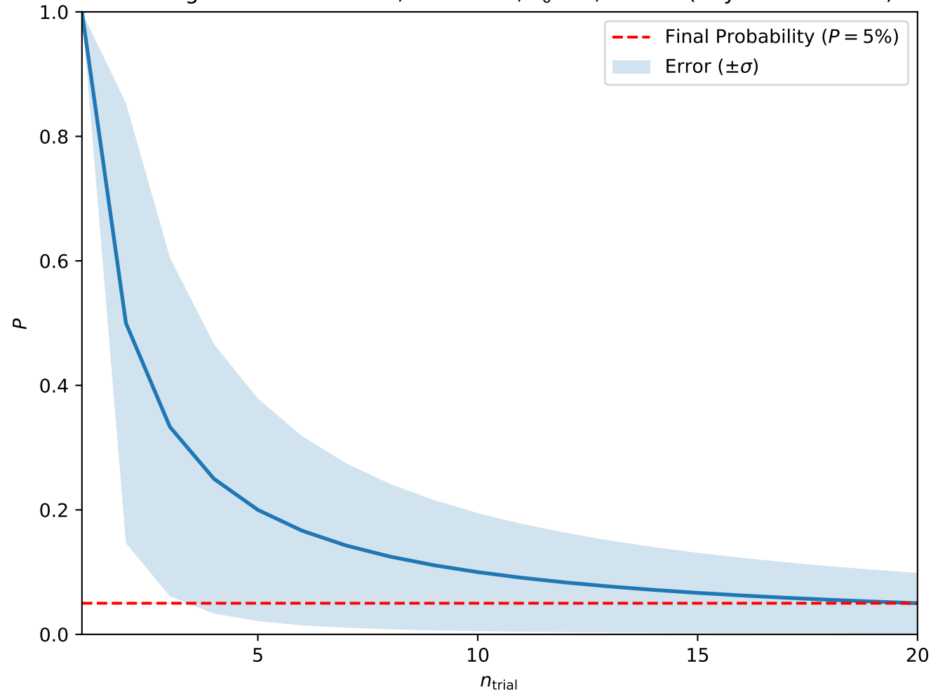
Convergence at A = 0.325, H = 0.275, T_0 = 3, w = 10 (Skyrmion Lattice)
