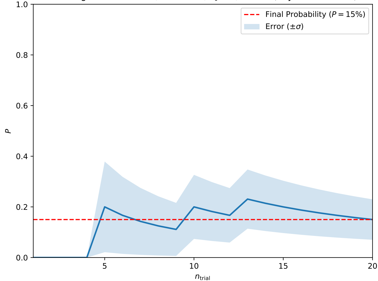
Convergence at A = 0.3, H = 0.275, T_0 = 3, w = 10 (Skyrmion Lattice)
