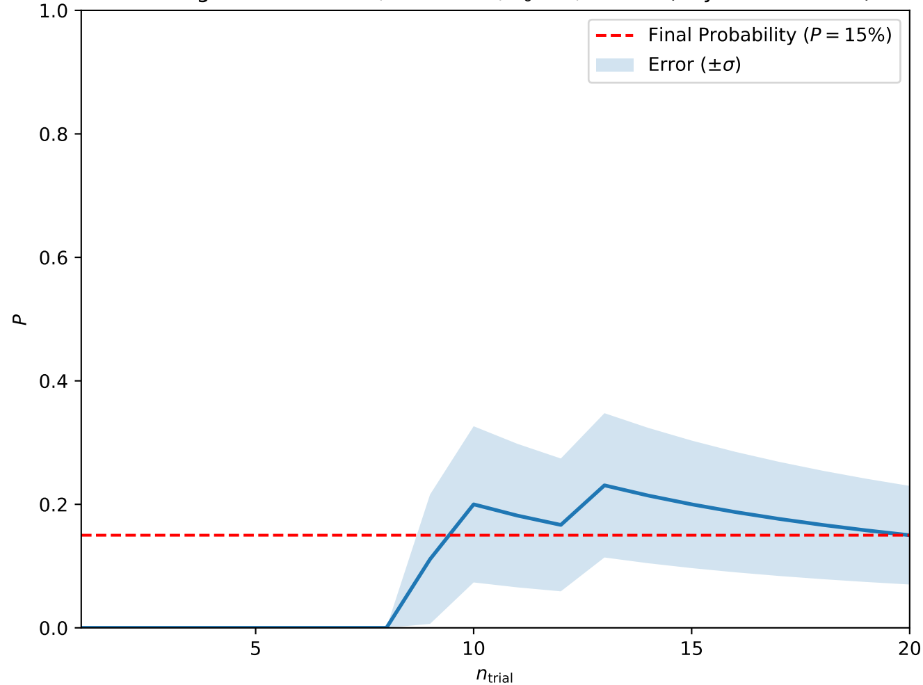
Convergence at A = 0.3, H = 0.325, T_0 = 3, w = 10 (Skyrmion Lattice)
