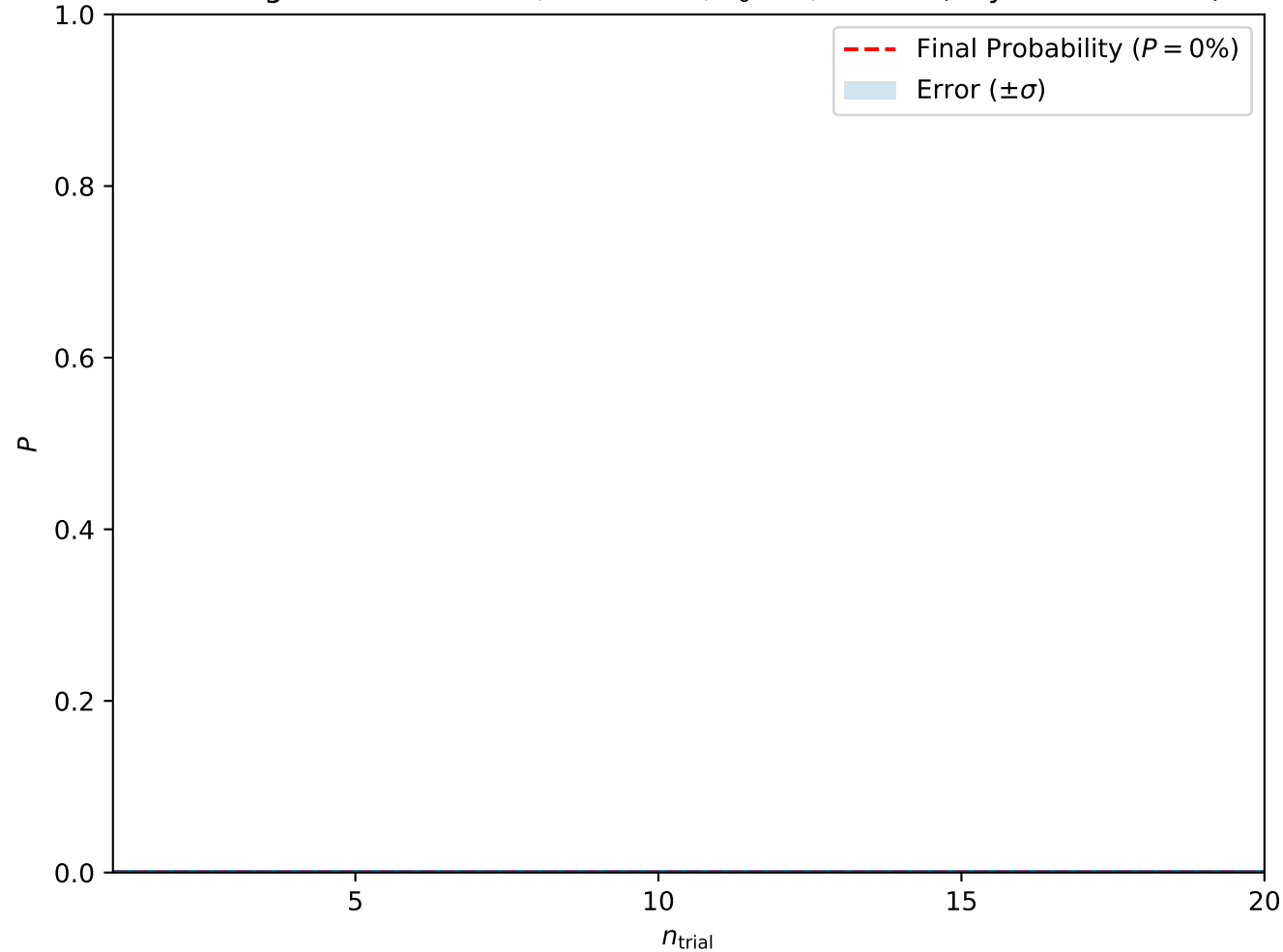
Convergence at A = 0.45, H = 0.375, T_0 = 3, w = 10 (Skyrmion Lattice)
