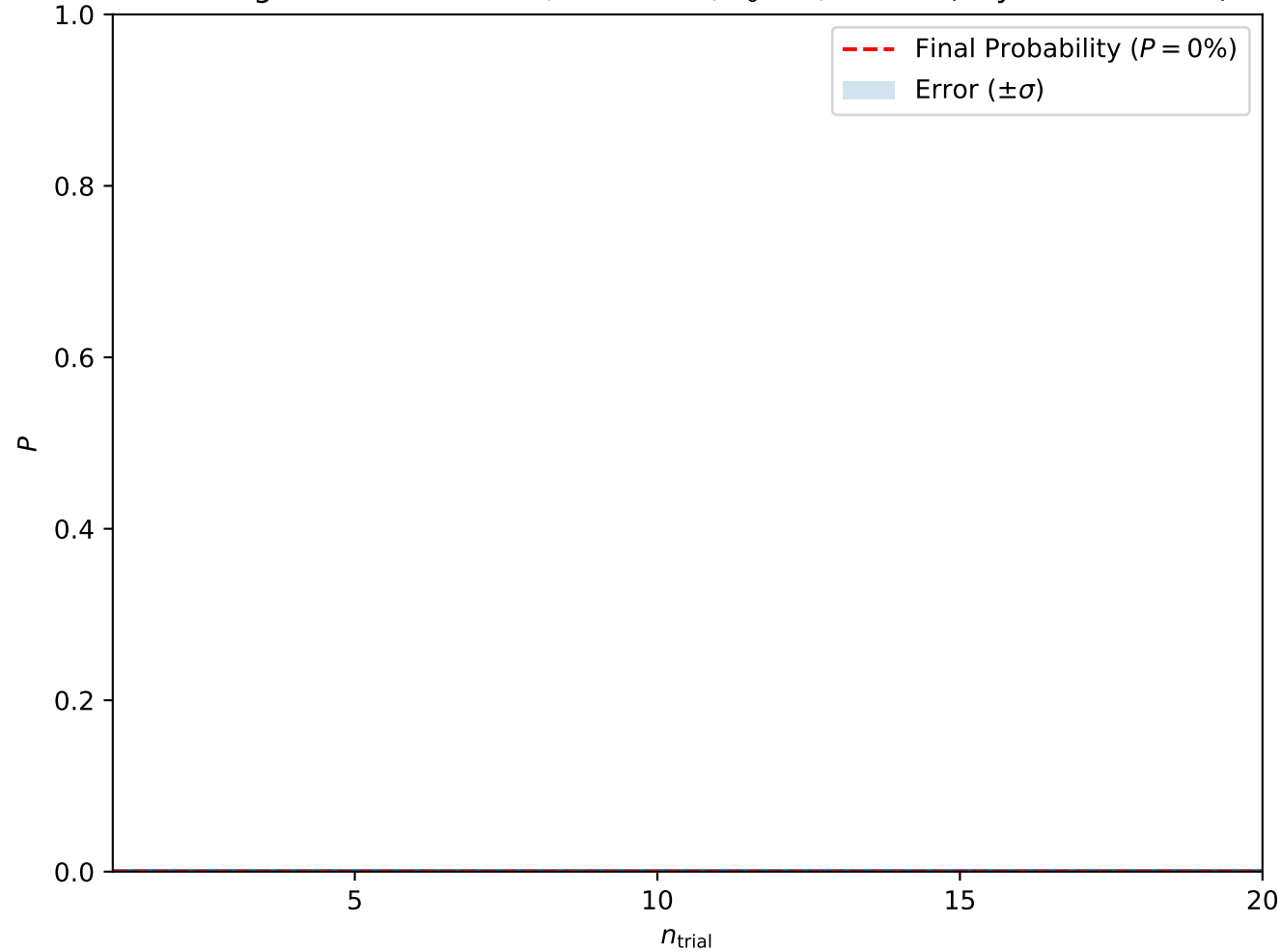
Convergence at A = 0.475, H = 0.325, T_0 = 3, w = 10 (Skyrmion Lattice)
