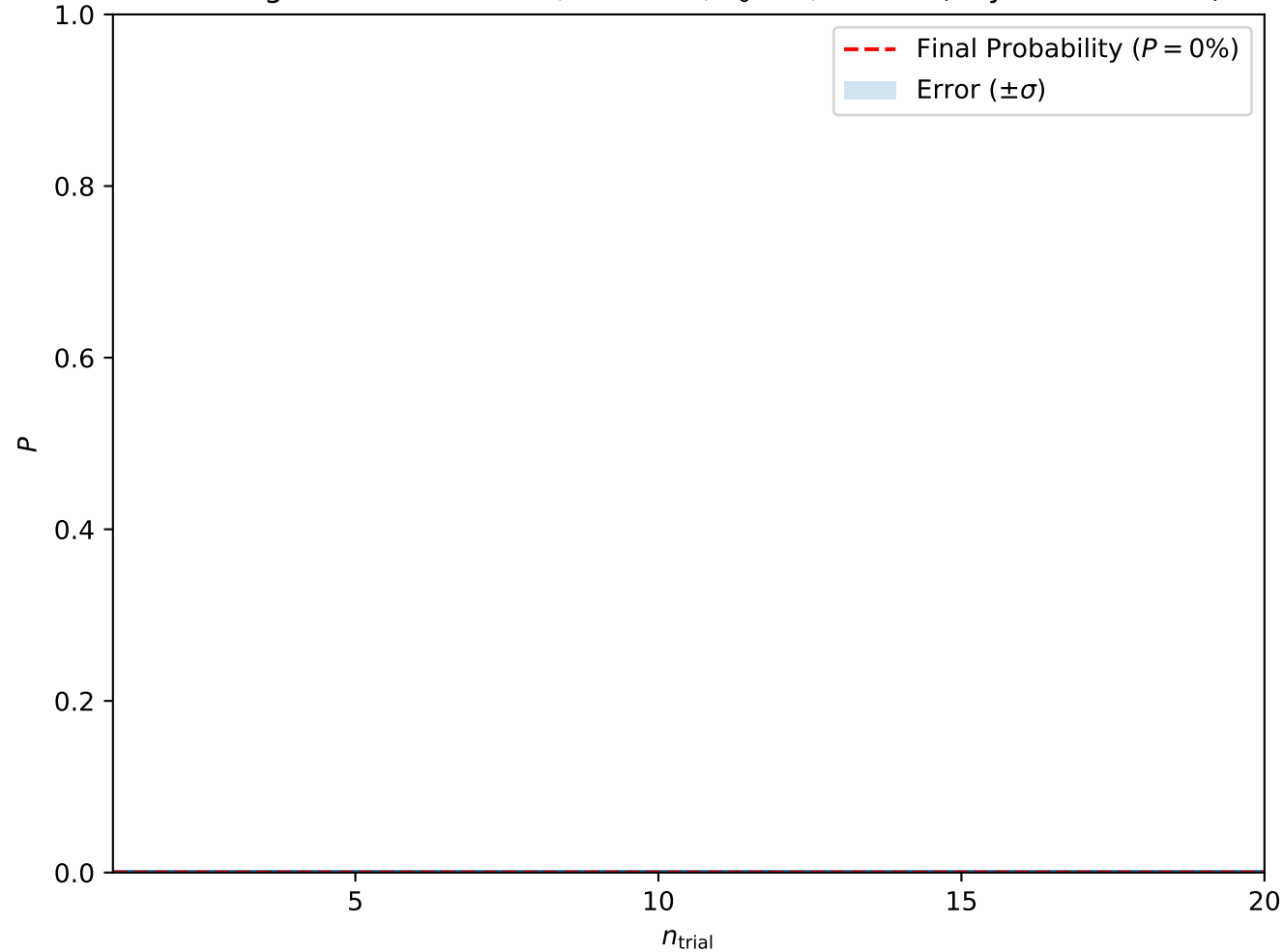
Convergence at A = 0.475, H = 0.35, T_0 = 3, w = 10 (Skyrmion Lattice)
