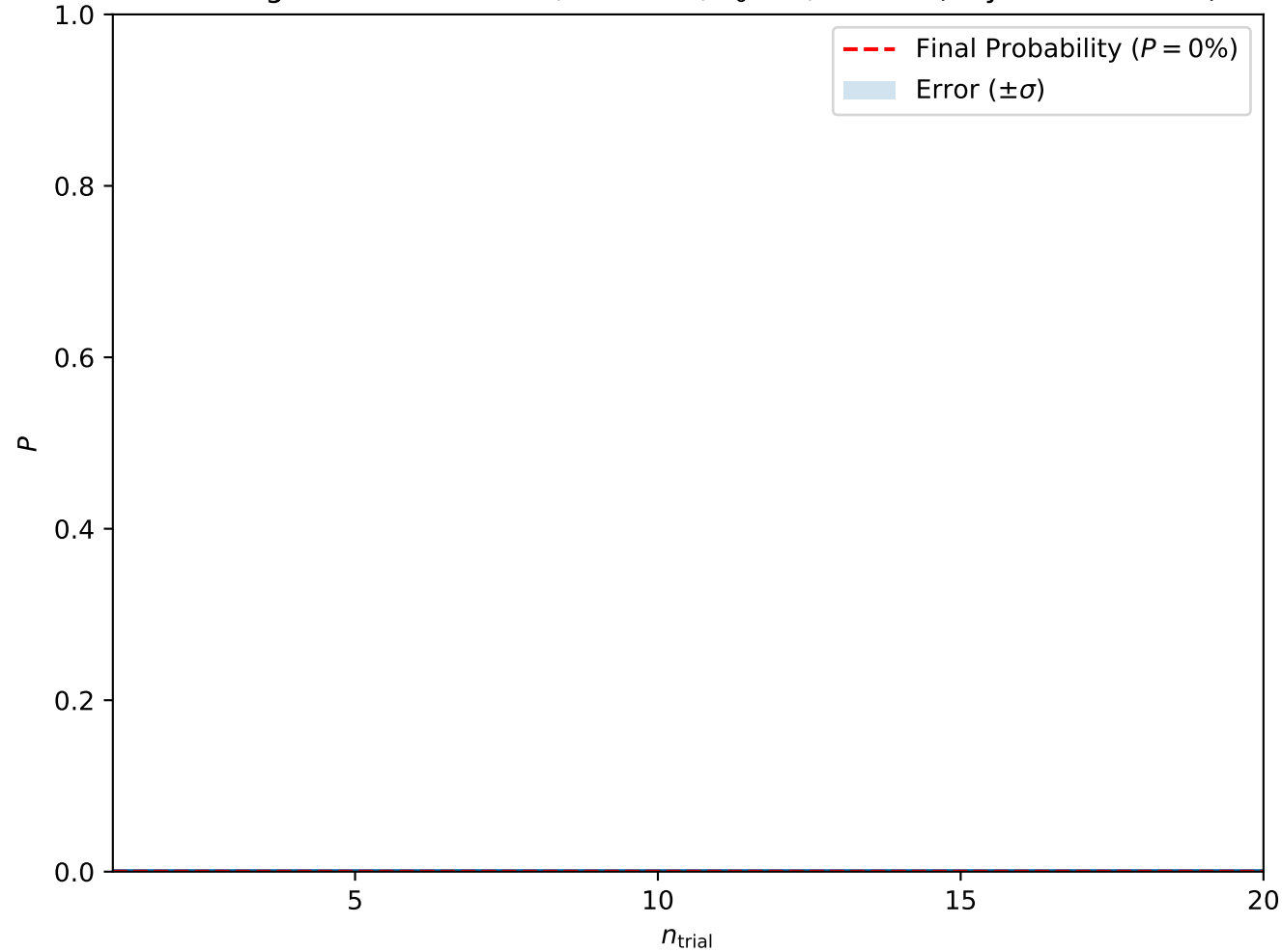
Convergence at A = 0.575, H = 0.25, T_0 = 3, w = 10 (Skyrmion Lattice)
