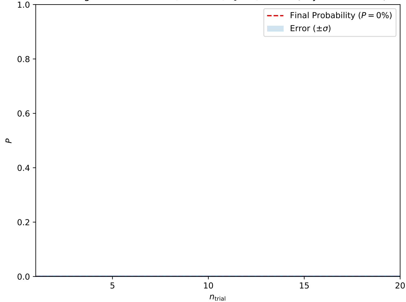
Convergence at A = 0.575, H = 0.55, T_0 = 3, w = 10 (Skyrmion Lattice)
