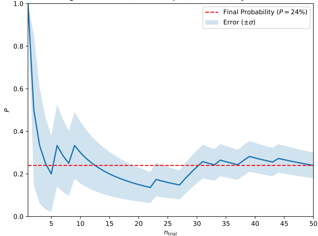
Convergence at A = 0.1, H = 0.3, T_0 = 1, w = 1.25 (Skyrmion Lattice)
