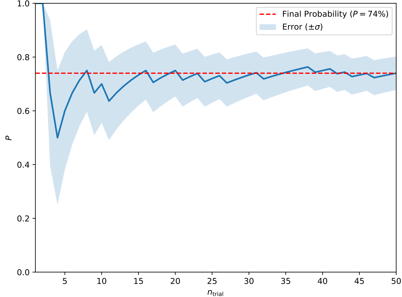
Convergence at A = 0.1, H = 0.3, T_0 = 1, w = 10 (Skyrmion Lattice)
