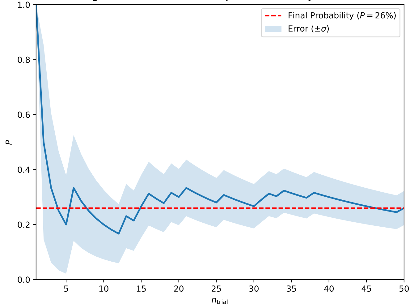
Convergence at A = 0.1, H = 0.3, T_0 = 1, w = 2.5 (Skyrmion Lattice)
