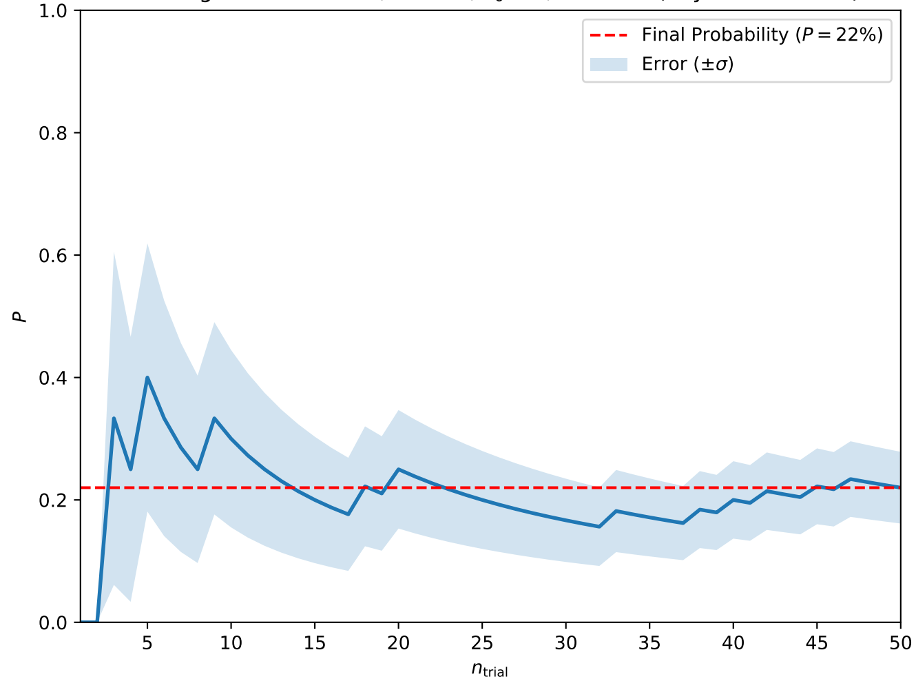
Convergence at A = 0.1, H = 0.3, T_0 = 3, w = 1.25 (Skyrmion Lattice)
