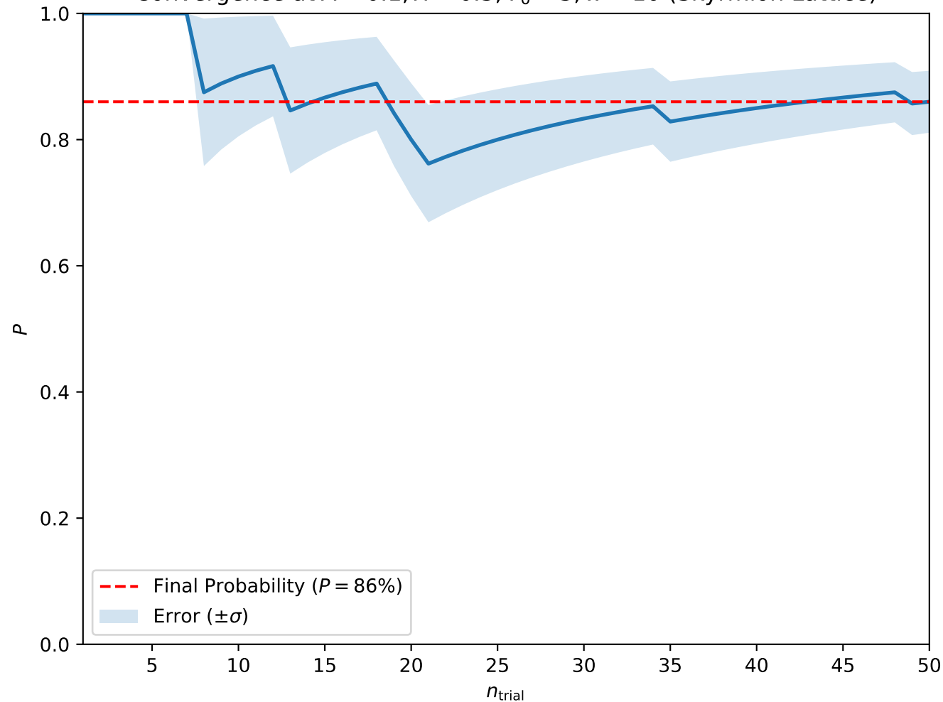
Convergence at A = 0.1, H = 0.3, T_0 = 3, w = 10 (Skyrmion Lattice)
