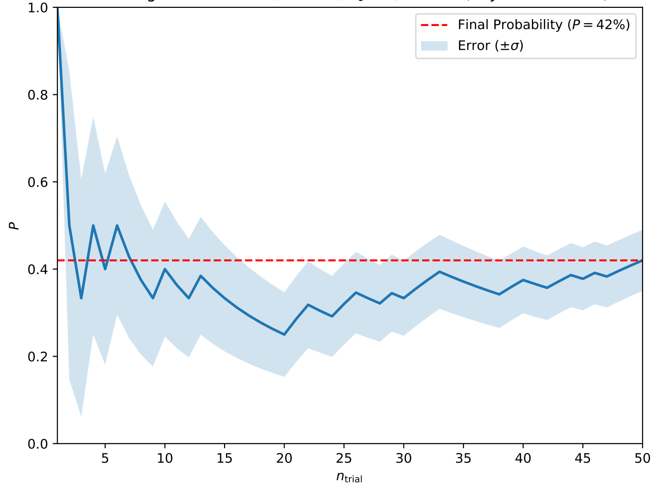
Convergence at A = 0.1, H = 0.3, T_0 = 3, w = 2.5 (Skyrmion Lattice)
