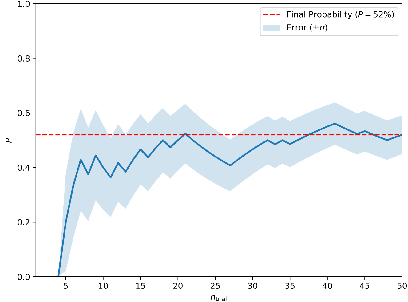
Convergence at A = 0.1, H = 0.3, T_0 = 3, w = 5 (Skyrmion Lattice)
