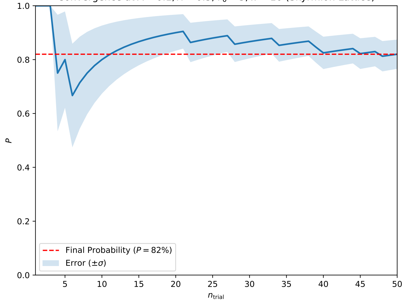
Convergence at A = 0.1, H = 0.3, T_0 = 5, w = 10 (Skyrmion Lattice)
