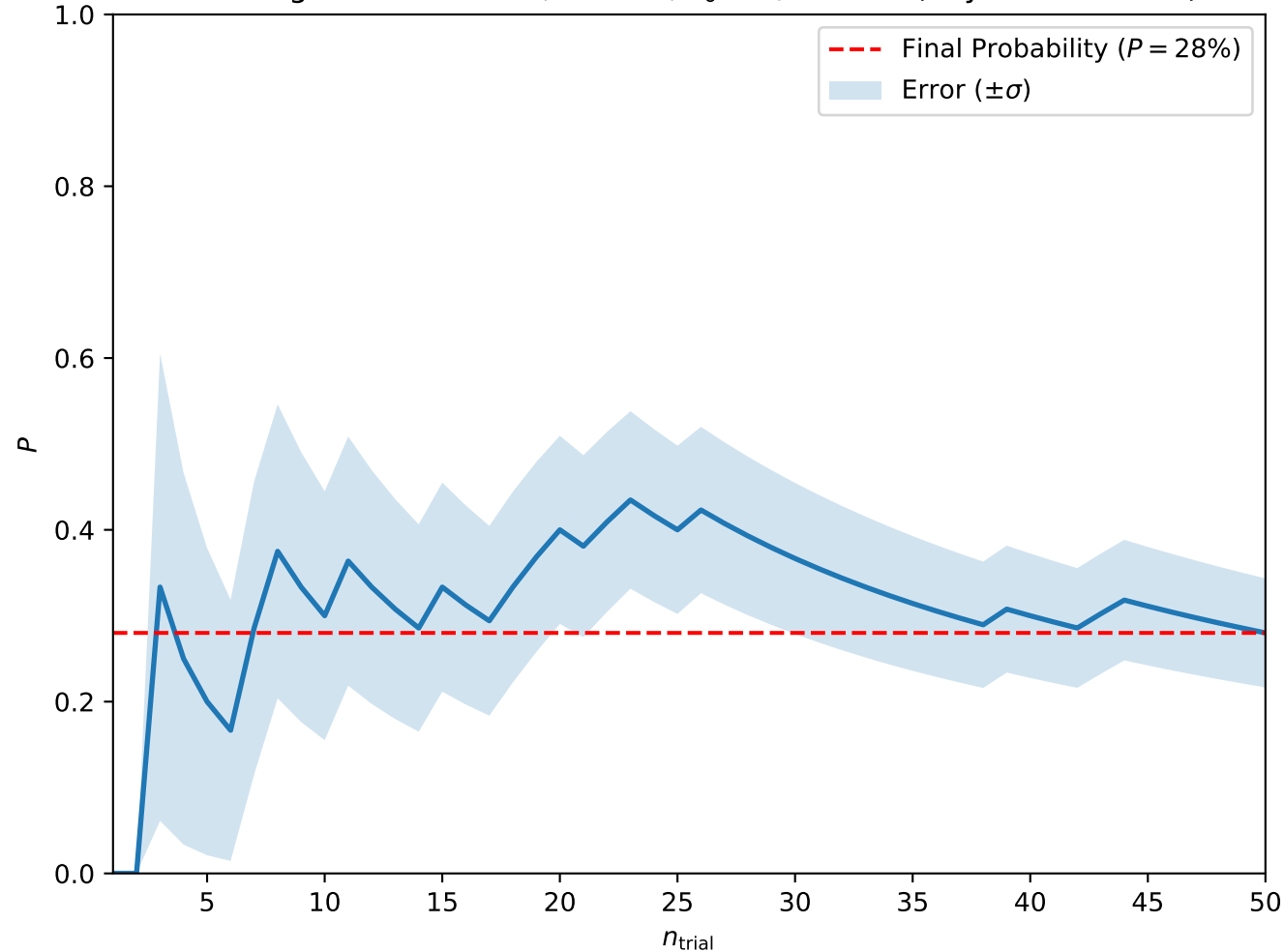
Convergence at A = 0.1, H = 0.3, T_0 = 5, w = 2.5 (Skyrmion Lattice)
