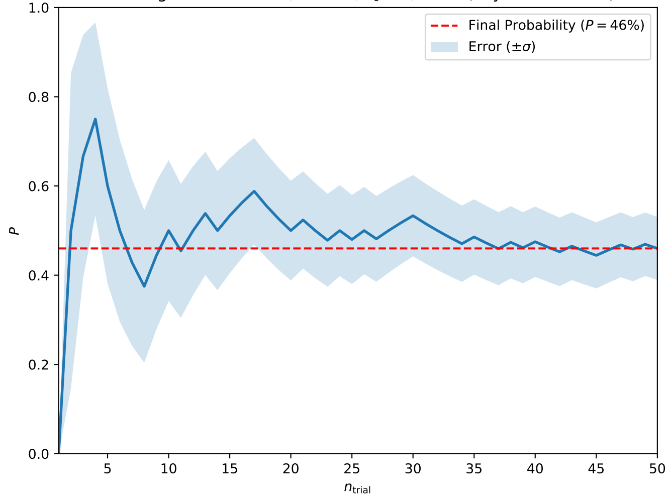
Convergence at A = 0.1, H = 0.3, T_0 = 5, w = 5 (Skyrmion Lattice)
