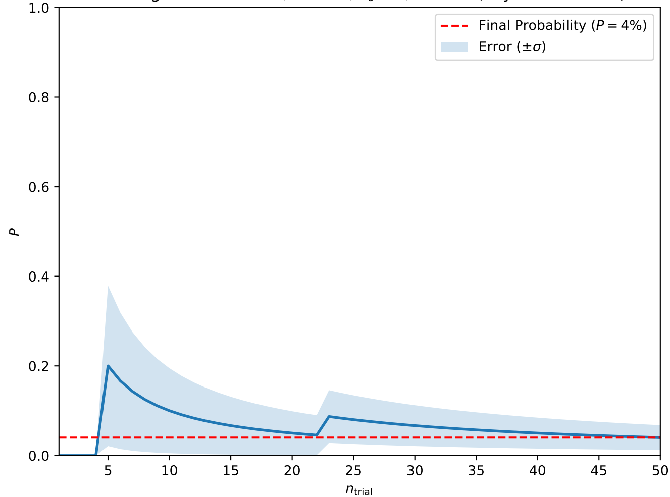
Convergence at A = 0.1, H = 0.4, T_0 = 1, w = 2.5 (Skyrmion Lattice)
