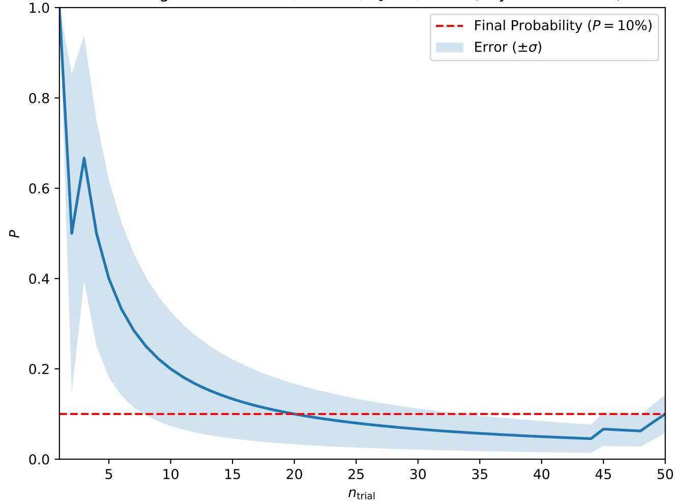
Convergence at A = 0.1, H = 0.4, T_0 = 1, w = 5 (Skyrmion Lattice)
