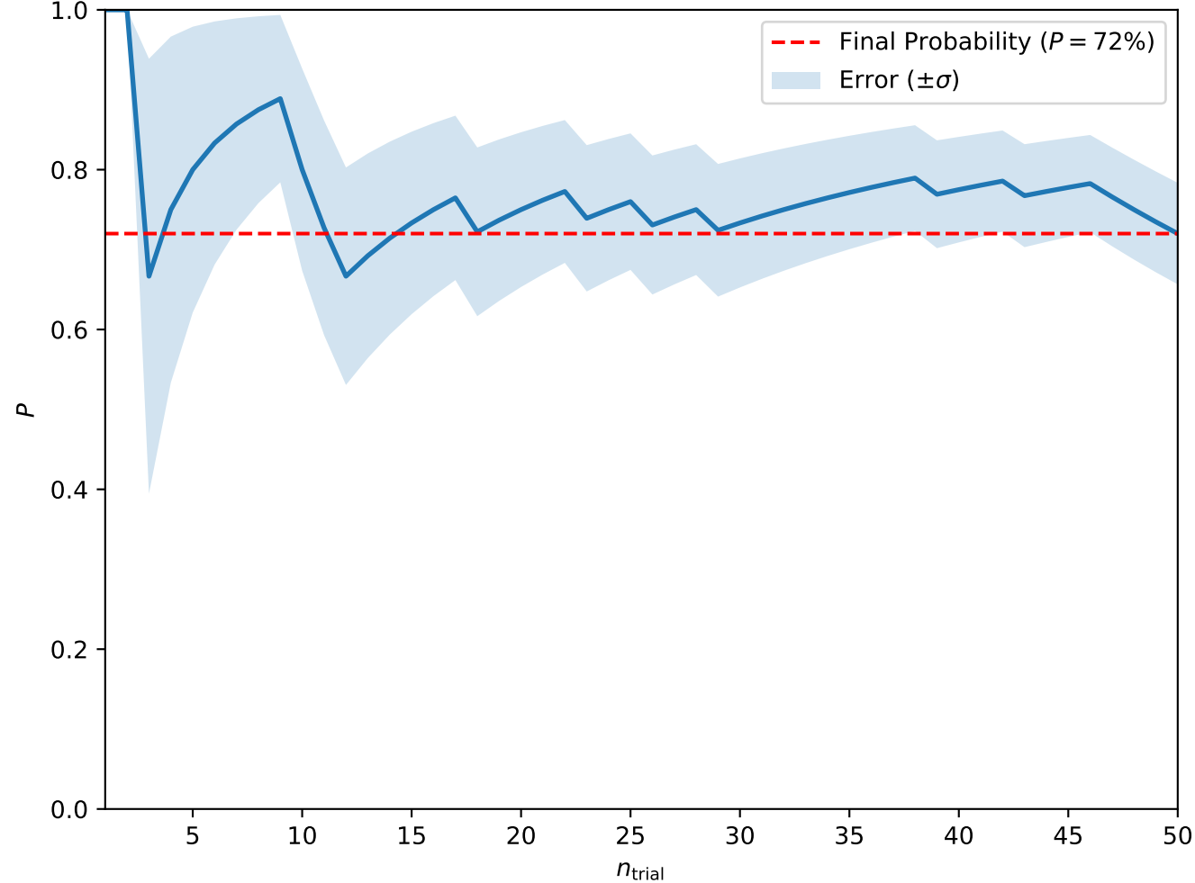
Convergence at A = 0.1, H = 0.4, T_0 = 3, w = 10 (Skyrmion Lattice)
