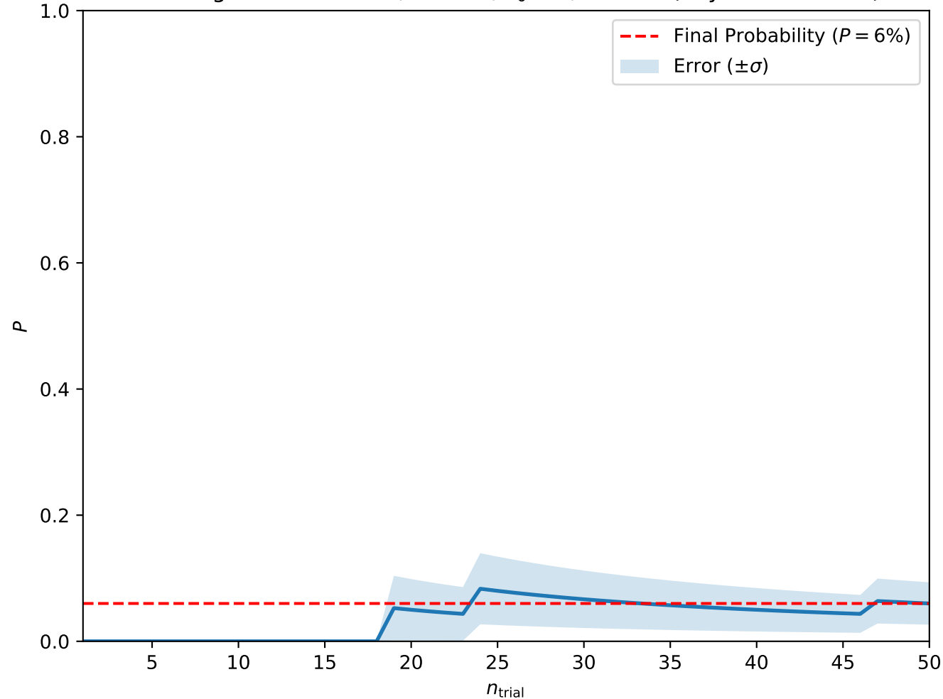
Convergence at A = 0.1, H = 0.4, T_0 = 3, w = 2.5 (Skyrmion Lattice)
