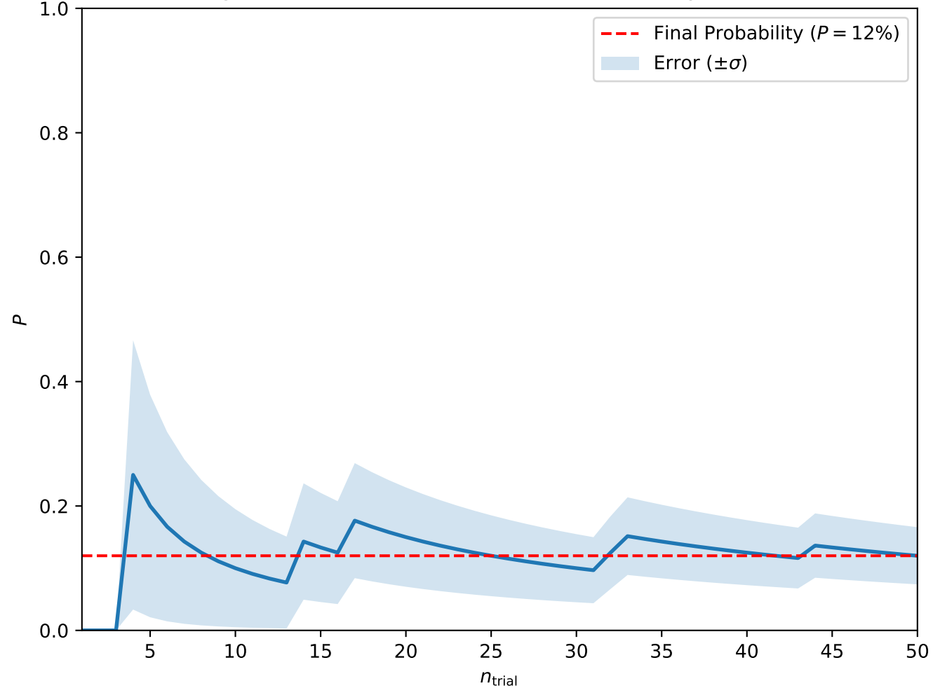
Convergence at A = 0.1, H = 0.4, T_0 = 3, w = 5 (Skyrmion Lattice)
