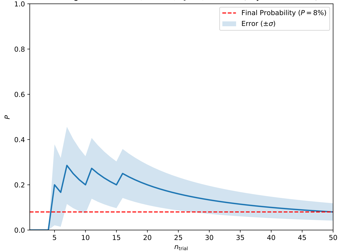
Convergence at A = 0.1, H = 0.4, T_0 = 5, w = 1.25 (Skyrmion Lattice)
