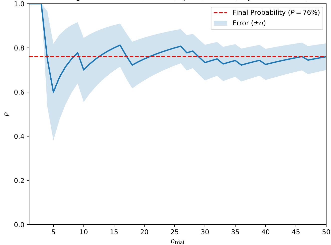
Convergence at A = 0.1, H = 0.4, T_0 = 5, w = 10 (Skyrmion Lattice)
