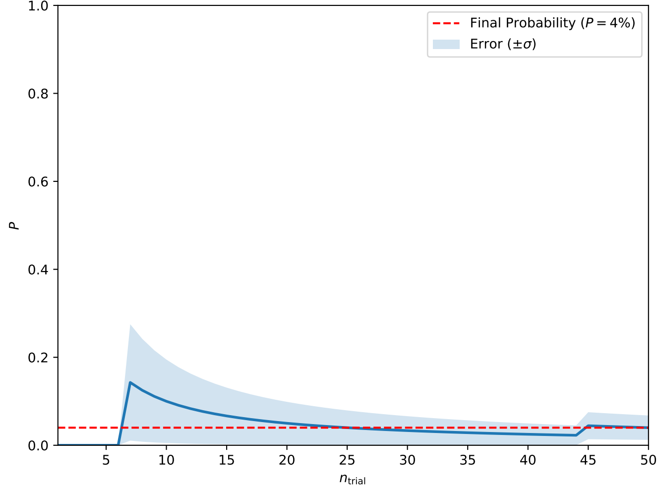
Convergence at A = 0.1, H = 0.4, T_0 = 5, w = 2.5 (Skyrmion Lattice)
