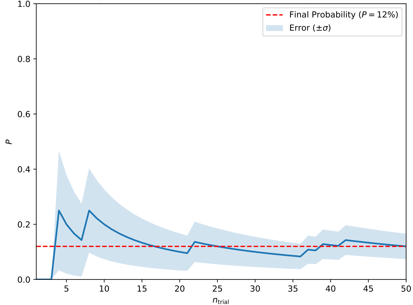
Convergence at A = 0.1, H = 0.4, T_0 = 5, w = 5 (Skyrmion Lattice)
