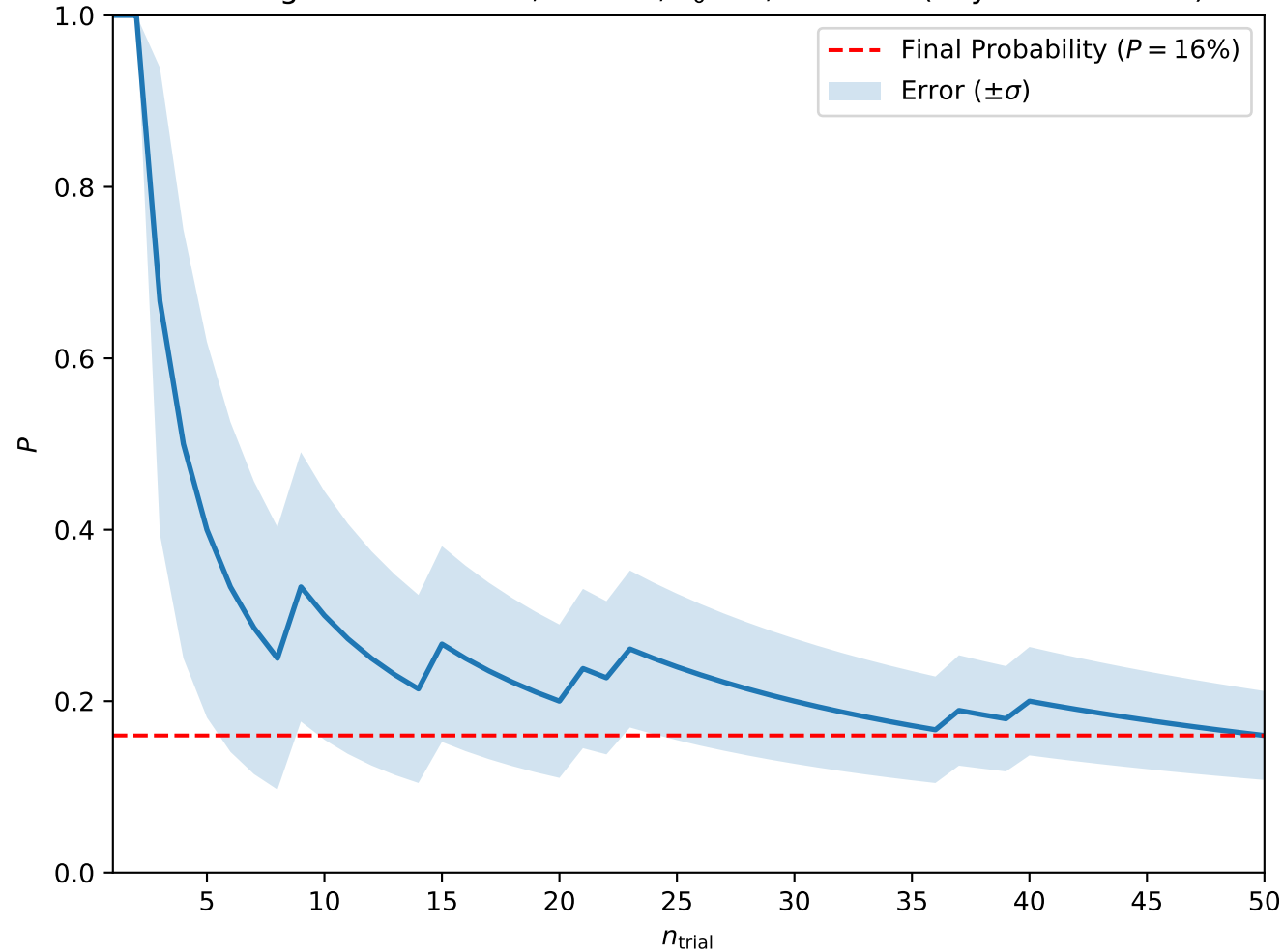
Convergence at A = 0.2, H = 0.3, T_0 = 1, w = 1.25 (Skyrmion Lattice)
