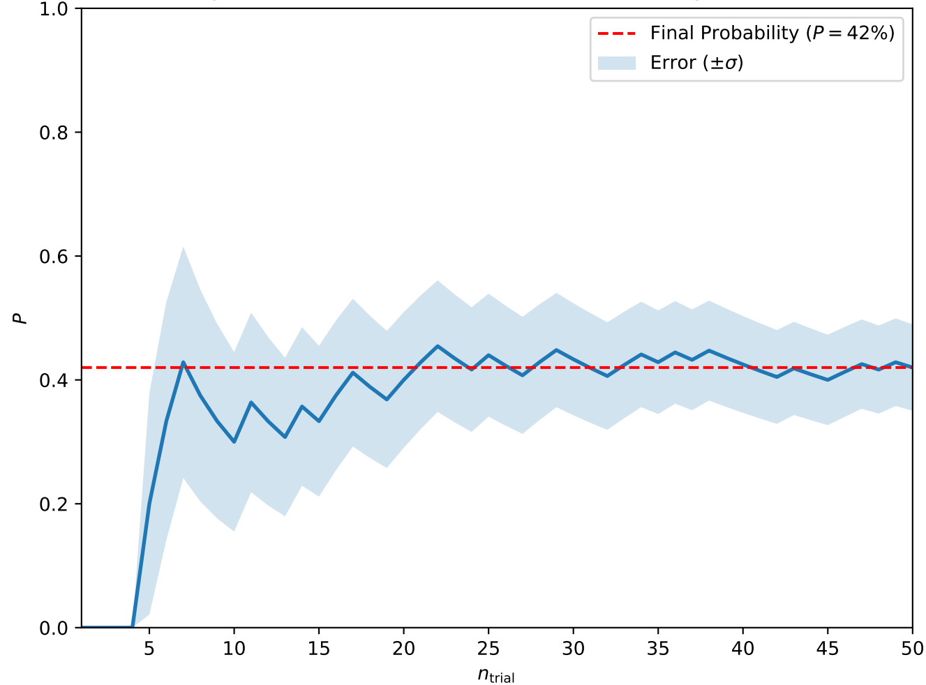
Convergence at A = 0.2, H = 0.3, T_0 = 1, w = 2.5 (Skyrmion Lattice)
