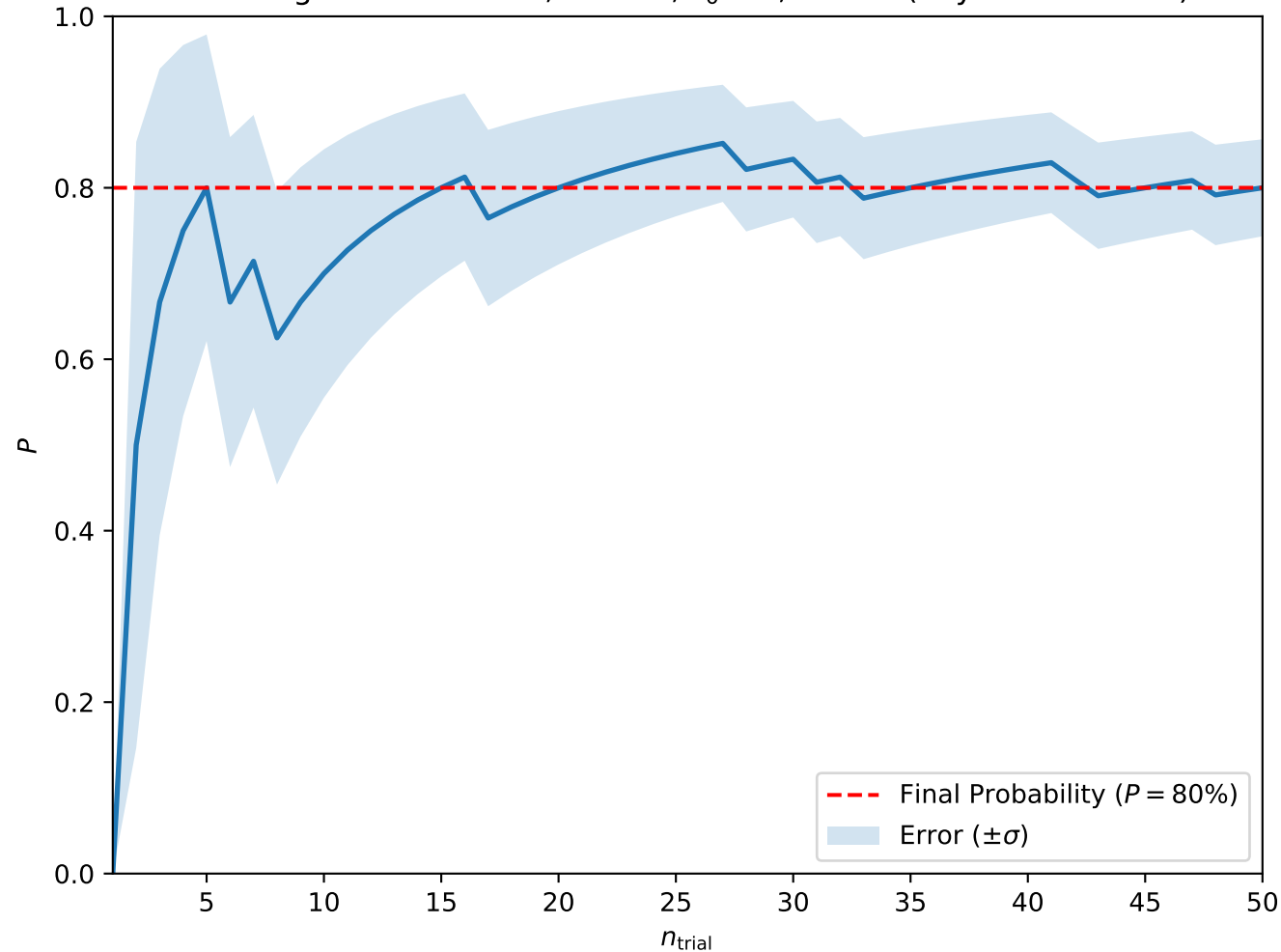
Convergence at A = 0.2, H = 0.3, T_0 = 3, w = 10 (Skyrmion Lattice)
