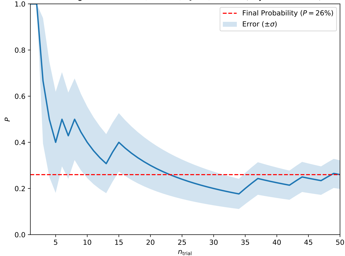
Convergence at A = 0.2, H = 0.3, T_0 = 3, w = 2.5 (Skyrmion Lattice)
