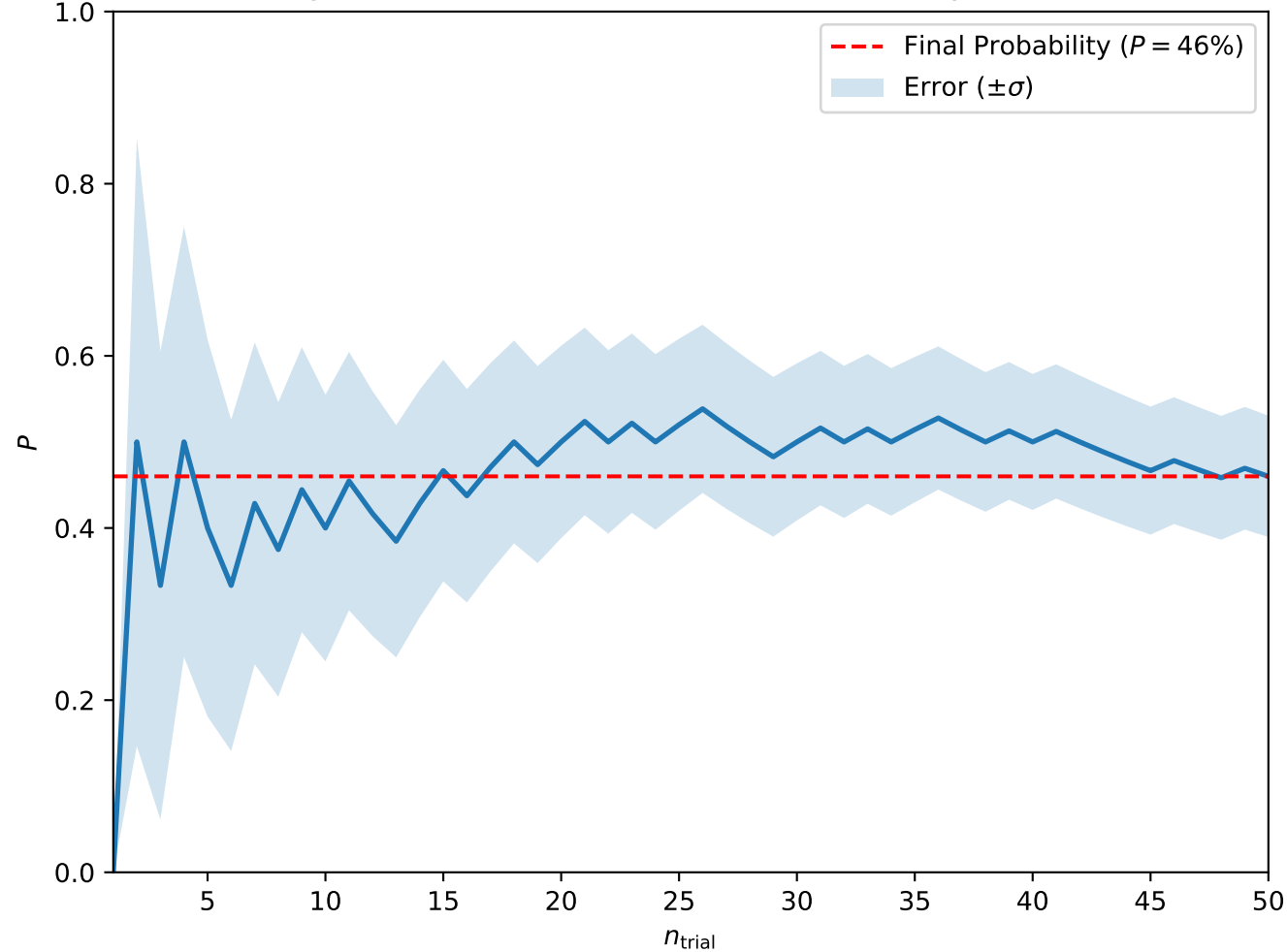
Convergence at A = 0.2, H = 0.3, T_0 = 3, w = 5 (Skyrmion Lattice)
