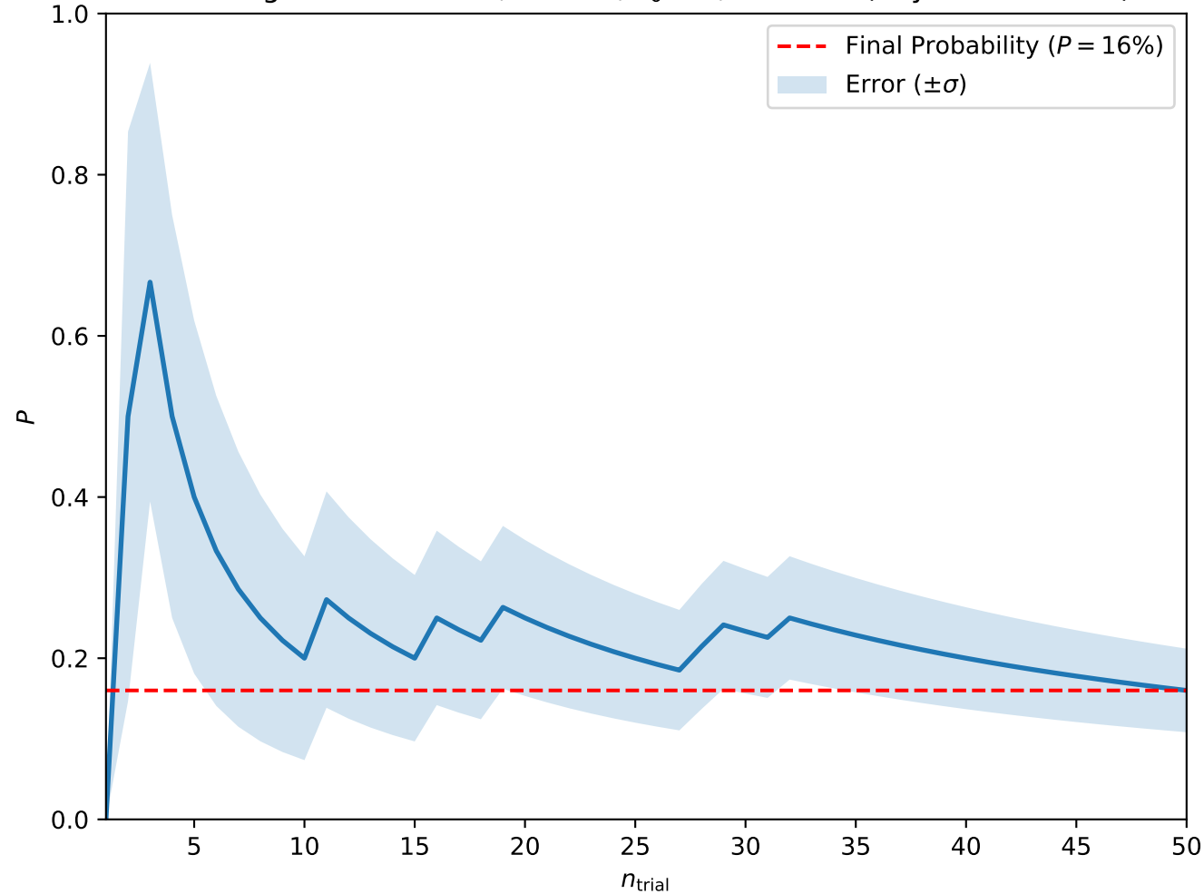
Convergence at A = 0.2, H = 0.3, T_0 = 5, w = 1.25 (Skyrmion Lattice)
