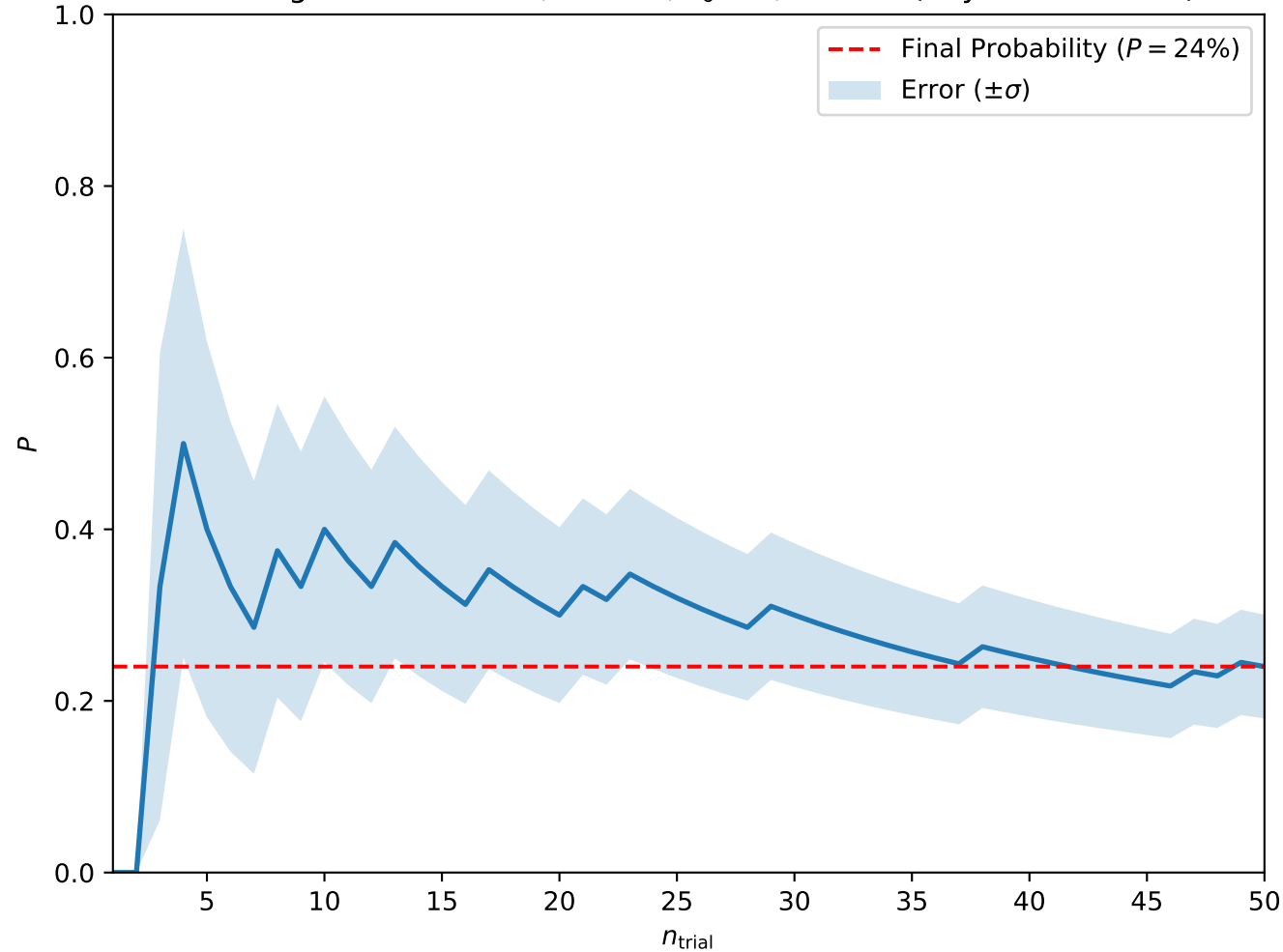
Convergence at A = 0.2, H = 0.3, T_0 = 5, w = 2.5 (Skyrmion Lattice)
