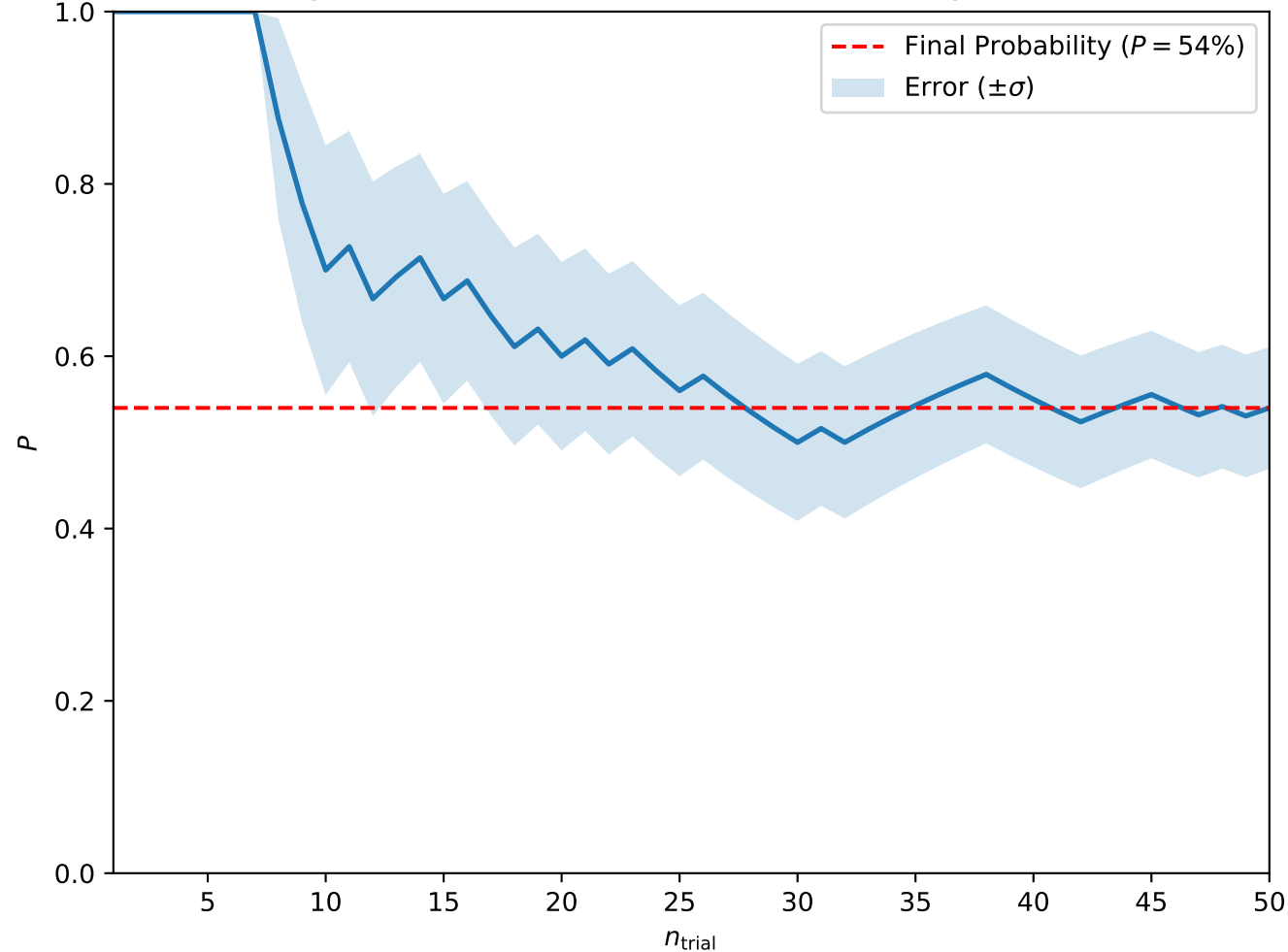
Convergence at A = 0.2, H = 0.3, T_0 = 5, w = 5 (Skyrmion Lattice)
