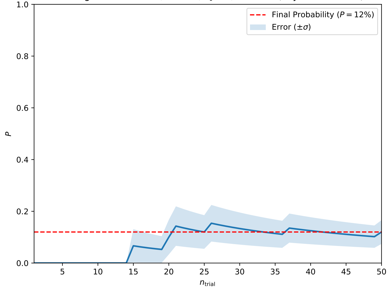
Convergence at A = 0.2, H = 0.4, T_0 = 1, w = 1.25 (Skyrmion Lattice)
