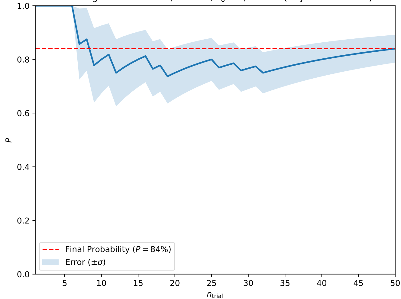
Convergence at A = 0.2, H = 0.4, T_0 = 1, w = 10 (Skyrmion Lattice)
