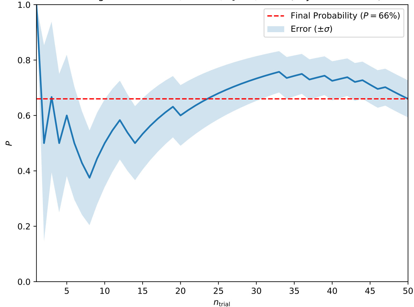
Convergence at A = 0.2, H = 0.4, T_0 = 1, w = 5 (Skyrmion Lattice)
