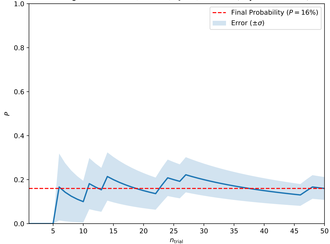
Convergence at A = 0.2, H = 0.4, T_0 = 3, w = 1.25 (Skyrmion Lattice)
